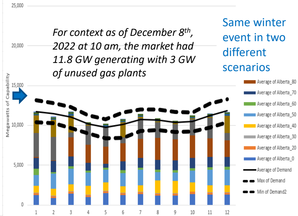
No WECC Buildout - Monthly Alberta Supply Compared to Demand
