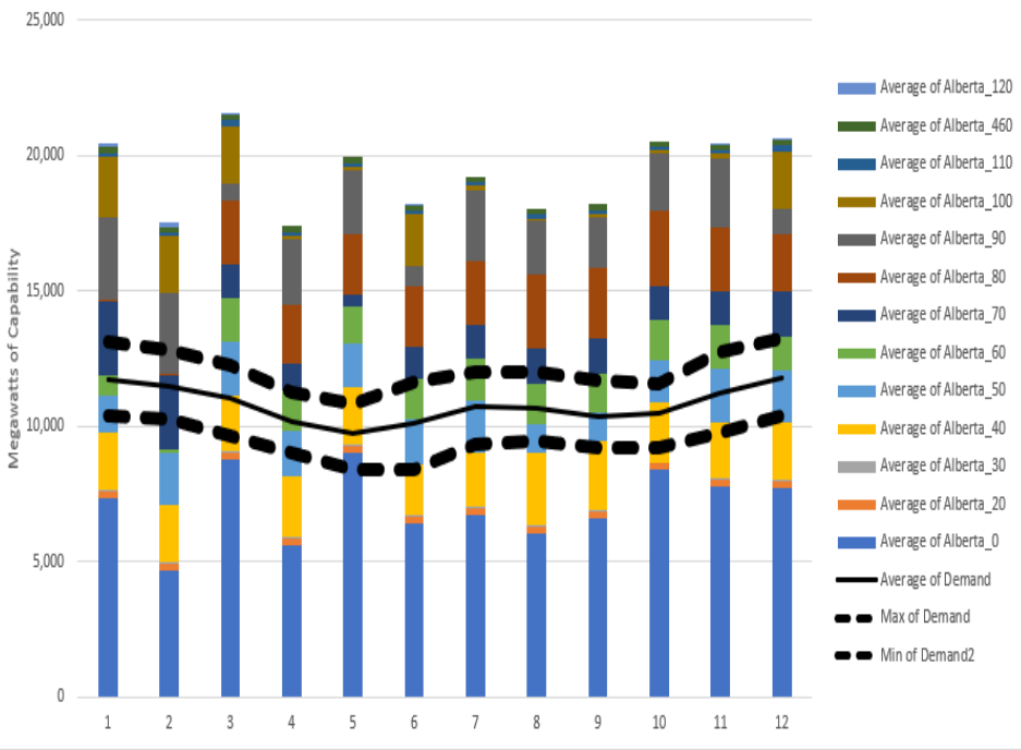
Baseline WECC Buildout - Monthly Alberta Supply Compared to Demand
